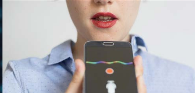
Voice Recognition
